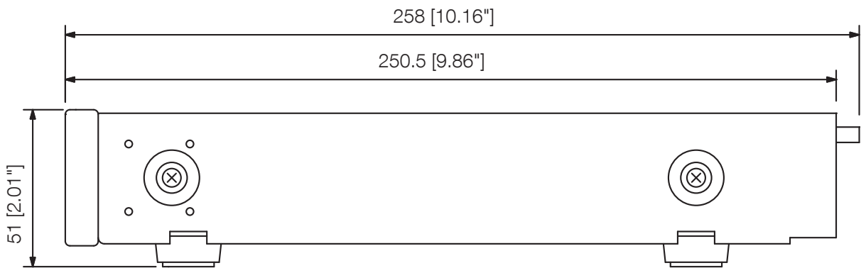
Side View
