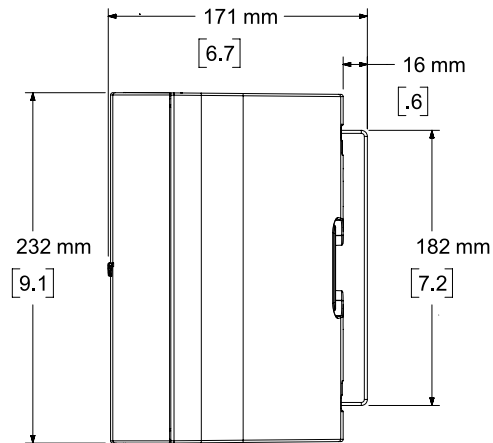
Right View
